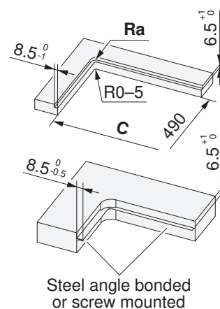
Detail Z
