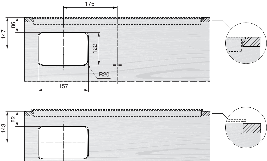
Installation for recirculation operation, unguided
