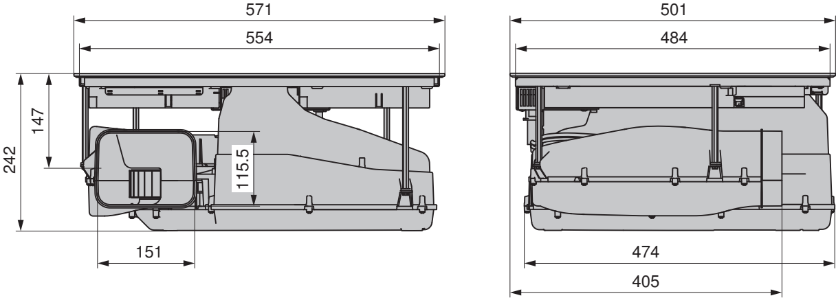
Installation for recirculation operation, unguided
